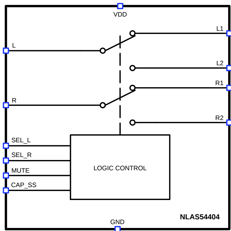
Figure 1. Block Diagram
