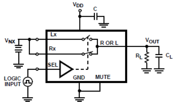
Figure 3. Switching Times
