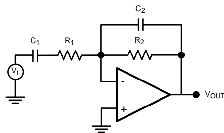
Figure 11. Bandpass Filter
