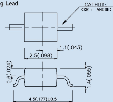
Subminiature Solid State Lamps Gull Wing Lead
