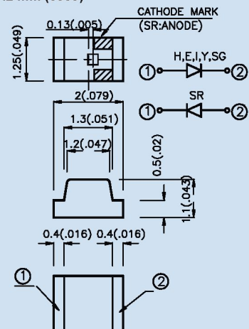
2.0 mm x 1.2 mm (0805)
