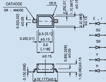
3.0 mm x 2.2 mm
