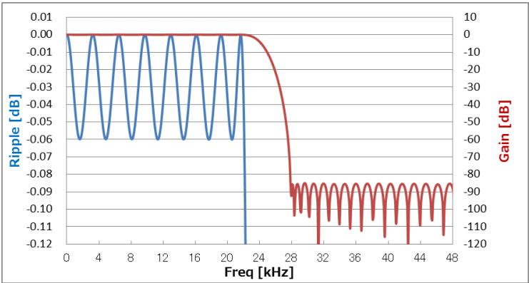
Figure 5. SHORT DELAY SHARP ROLL-OFF (fs=48kHz)
