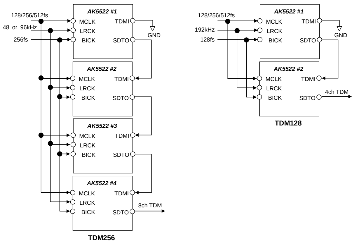
Figure 60. Cascade Connection
