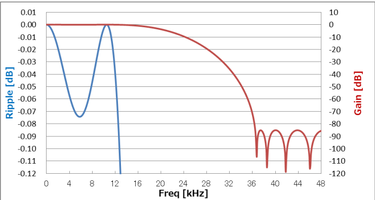
Figure 6. SHORT DELAY SLOW ROLL-OFF (fs=48kHz)
