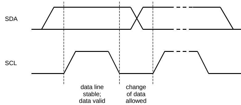
Figure 80. Bit Transfer on the I 2 C-Bus
