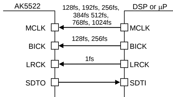
Figure 55. EXT Slave Mode (TDM128, TDM256 Output)
