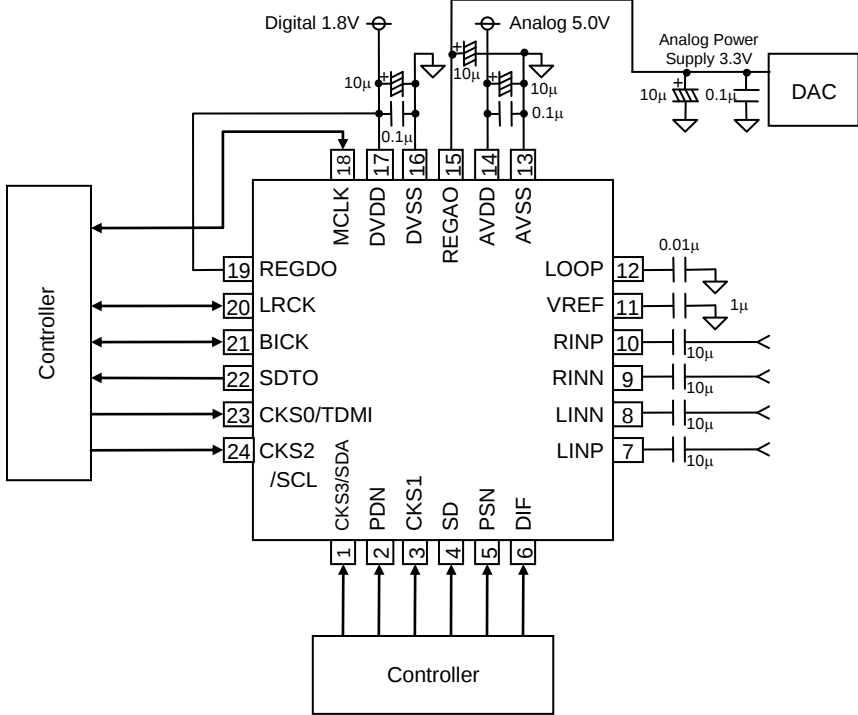
Figure 82. Typical Connection Diagram (Analog 5V, Digital I/O 1.8V)
