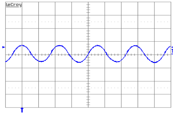
Figure 13. Input reflected ripple-current, i_c (200 mA/div.), measured at input terminals at full rated load current and V_{in} = 48\text{V} . Refer to Figure 11 for test setup. Time scale: 1 \mu\text{s}/\text{div} .
