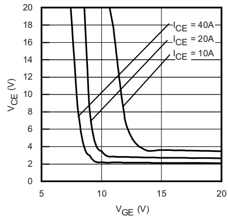
Fig. 9 - Typical V_{CE} vs. V_{GE} T_J = -40^\circ\text{C}
