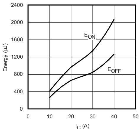
Fig. 13 - Typical Energy Loss vs. I_C T_J = 150^\circ\text{C} ; L = 1.4\text{ mH} ; V_{CE} = 400\text{ V} R_g = 5\ \Omega ; V_{GE} = 15\text{ V}
