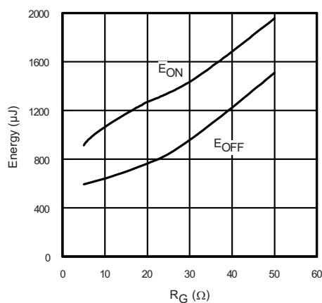
Fig. 15 - Typical Energy Loss vs. R_g T_J = 150^\circ\text{C} ; L = 1.4\text{ mH} ; V_{CE} = 400\text{ V} I_{CE} = 5.0\text{ A} ; V_{GE} = 15\text{ V}
