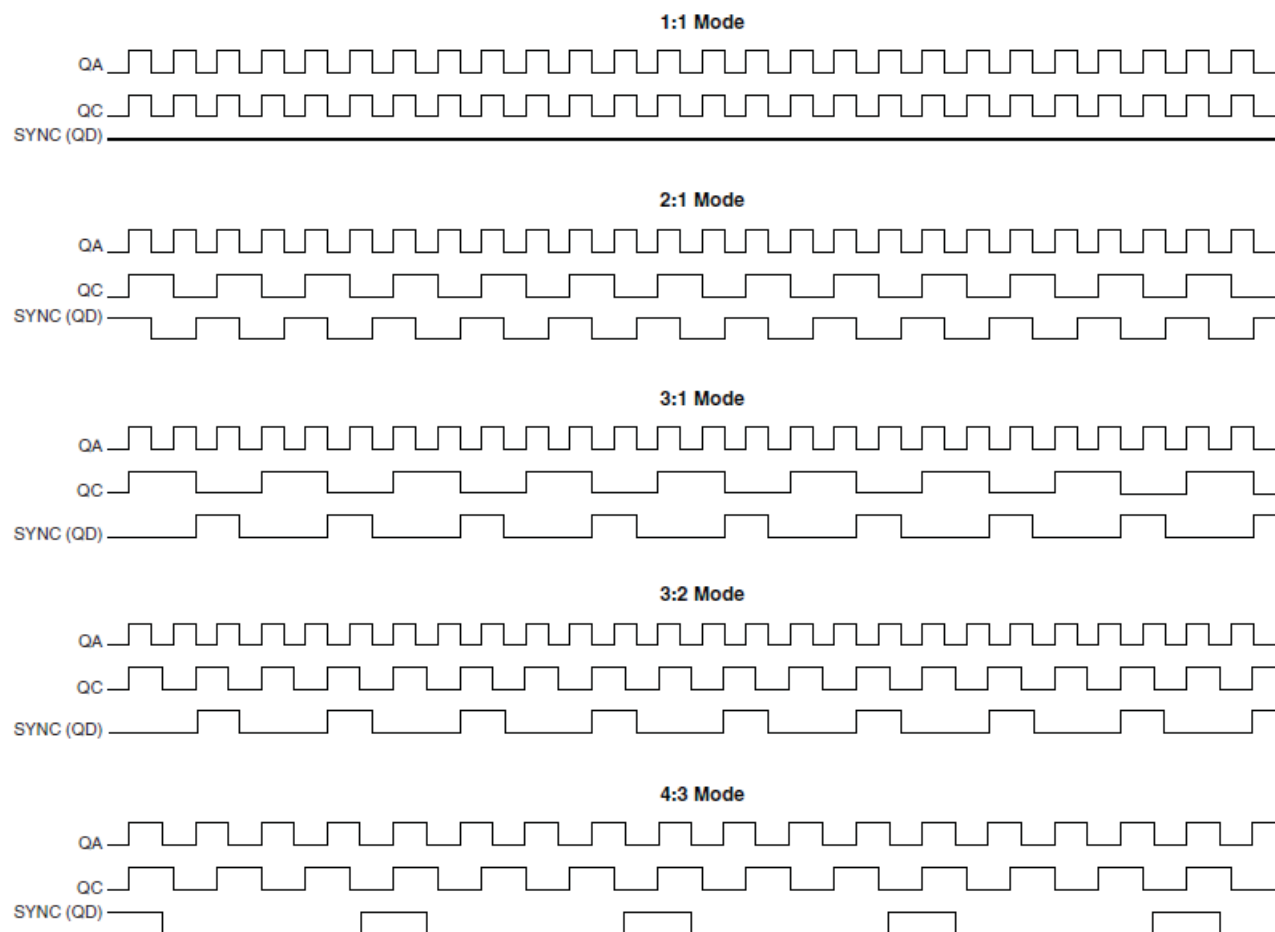
FIGURE 1. TIMING DIAGRAMS
