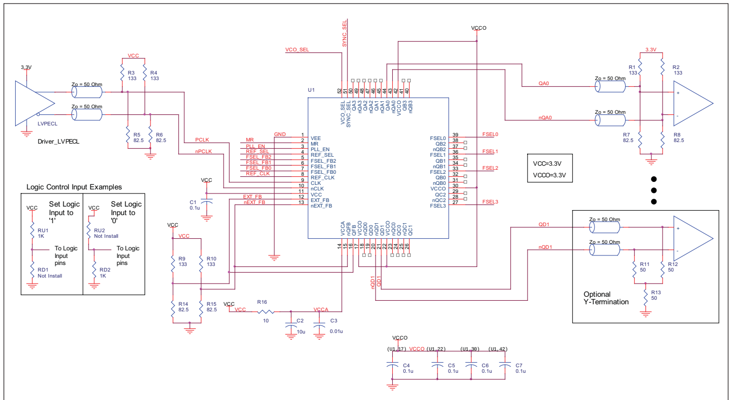
FIGURE 6. 873991-147 SCHMATIC LAYOUT
