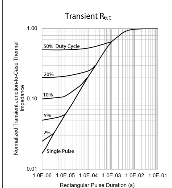
Figure 15: Transient Thermal Impedance 1.00 = Normalized DC thermal impedance
