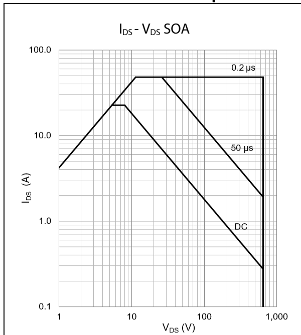
Figure 13: Safe Operating Area @ T_{case} = 25^\circ\text{C}
