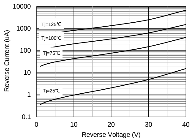
Fig.2 - Typical Reverse Leakage Characteristics (per diode)
