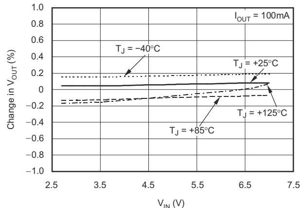
Figure 6-2. Line Regulation
