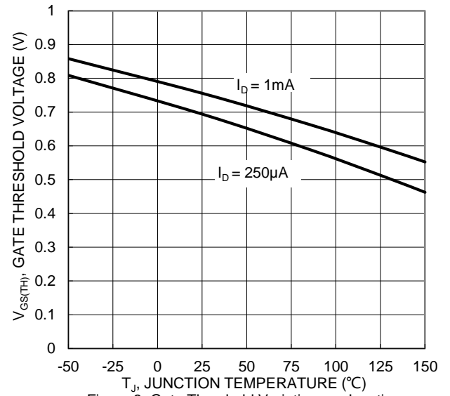
Figure 8. Gate Threshold Voltage vs. Junction Temperature
