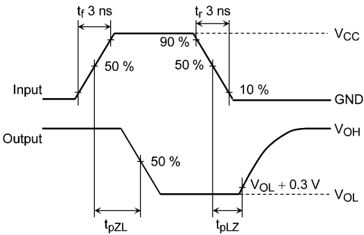
AC Waveform
