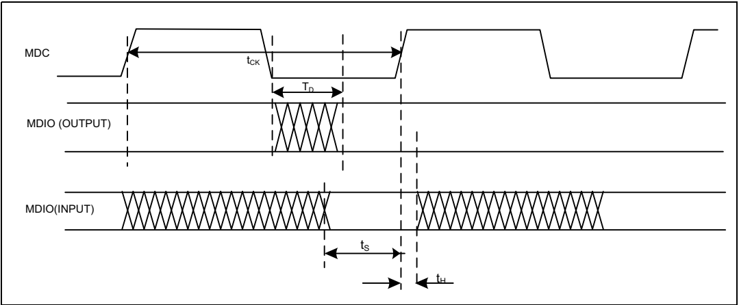
Figure 19. MDC waveform
