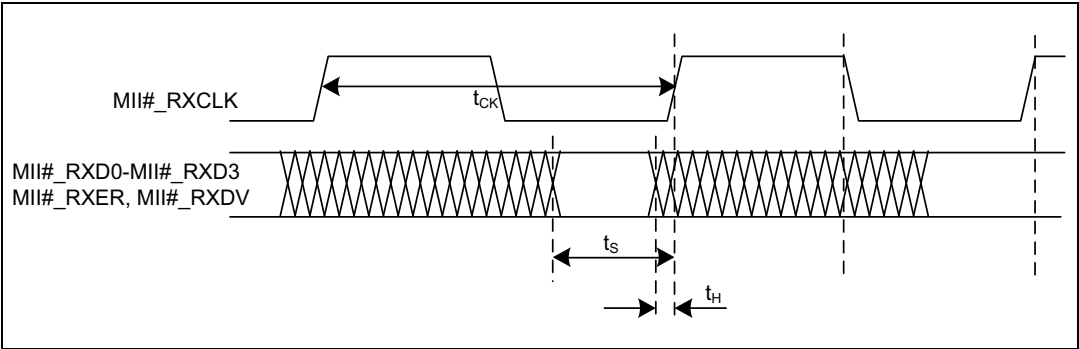
Figure 18. MII RX waveform
