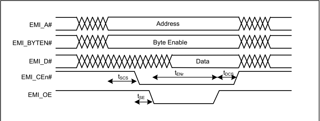
Figure 15. EMI read cycle waveform without acknowledgement on EMI_WAIT
