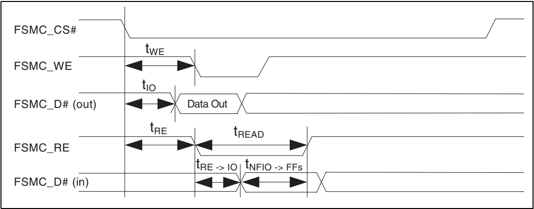
Figure 24. In/out data address signal waveform
