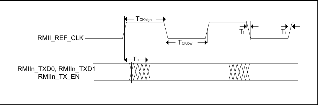
Figure 20. RMII TX waveform
