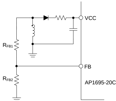
Figure 4. OVP Circuit
