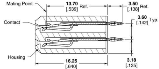
Section Y-Y
