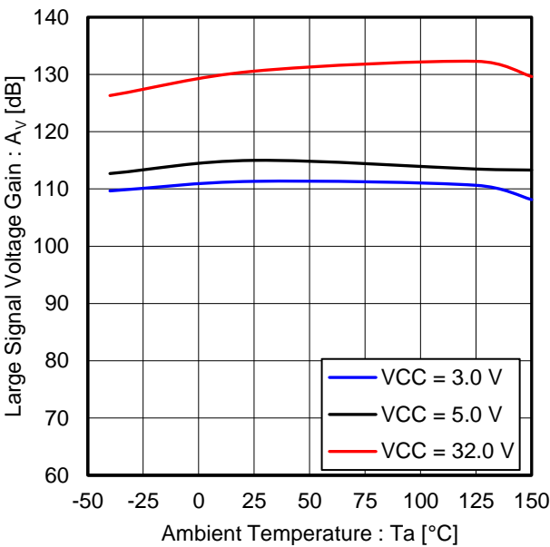
Figure 14. Large Signal Voltage Gain vs Ambient Temperature
