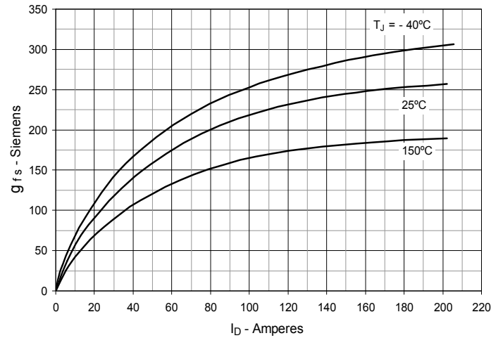
Fig. 8. Transconductance
