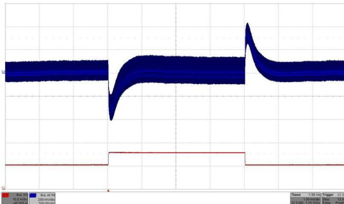
Fig. 24: Output voltage response to load current step change 50% - 75% - 50% (10.5A - 15.75A - 10.5A) with di/dt = 1A/\mu s at V_{IN} = 24V . Top trace (C4): Output voltage (200 mV/div.). Bottom trace (C3): Load current (10A/div.). C_O 470 \mu F /70m \Omega . Time: 1ms/div.
