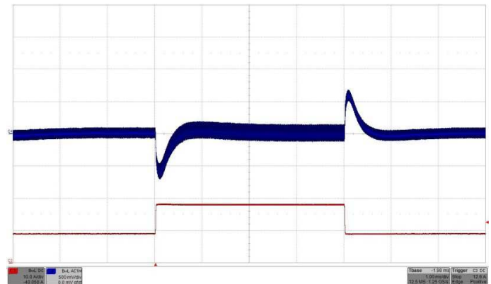
Fig. 31: Output voltage response to load current step change 50% - 100% - 50% (9A - 18A - 9A) with di/dt = 1A/\mu s at V_{IN} = 24V . Top trace (C4): Output voltage (500 mV/div.). Bottom trace (C3): Load current (10A/div.). C_O 470 \mu F /70m \Omega . Time: 1ms/div.
