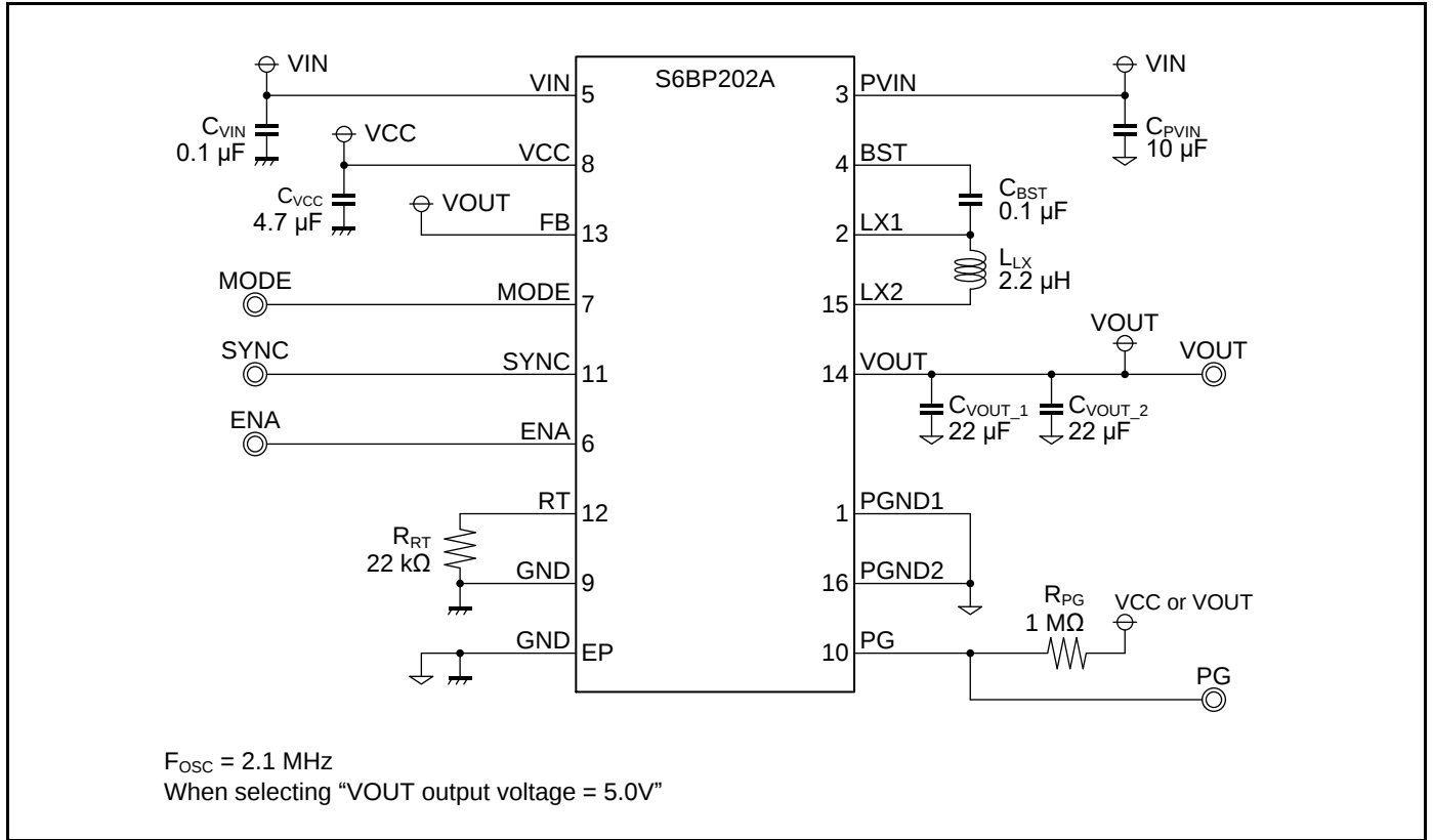
Figure 9-1 Application Circuit Example
