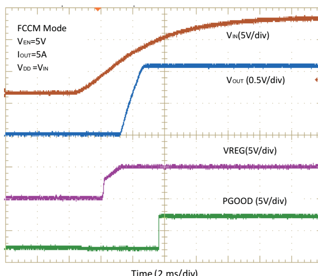
Figure 22. UVLO Start-Up
