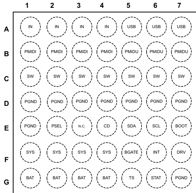
Figure 6-2. YFF Package WCSP 49 Pins Top View
