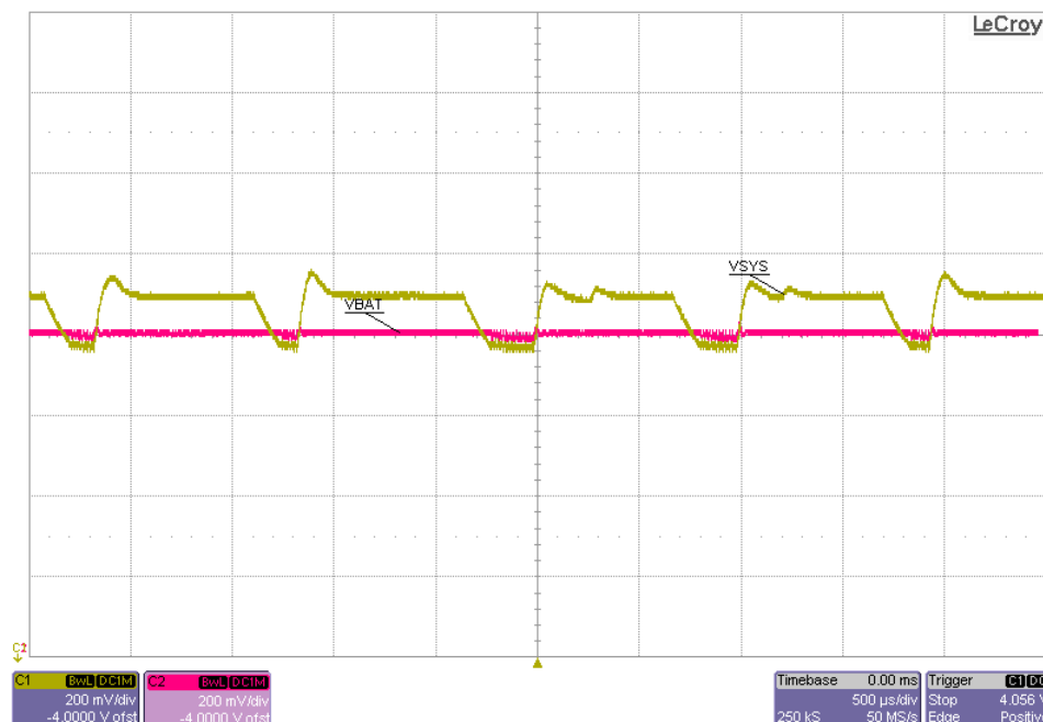
Figure 8-7. V(SYS) When Reverse Boost Prevention Circuit is Active
