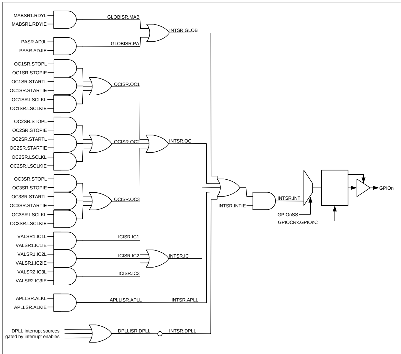
Figure 19 – Interrupt Structure
