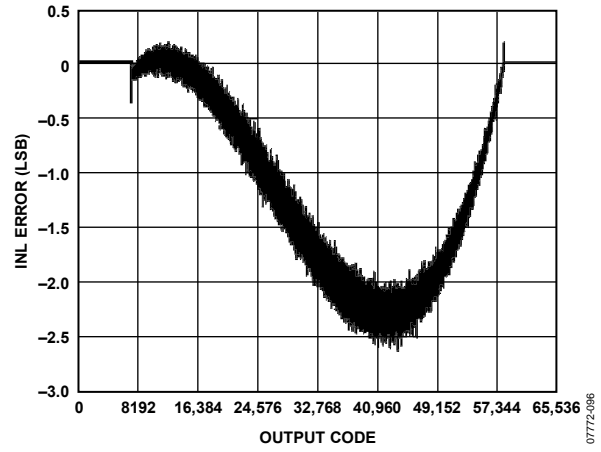
Figure 29. AD9262BCPZ-10 INL
