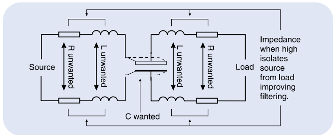
Figure 2: T-Network capacitor
