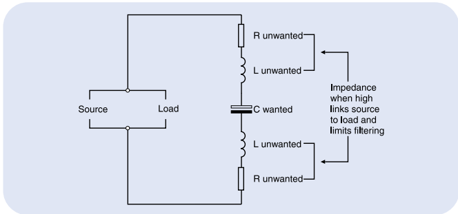
Figure 1: Conventional capacitor
