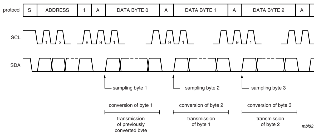
Fig 11. A/D conversion sequence
