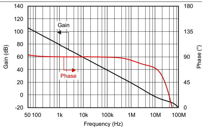
Figure 5. Gain and Phase vs Frequency
