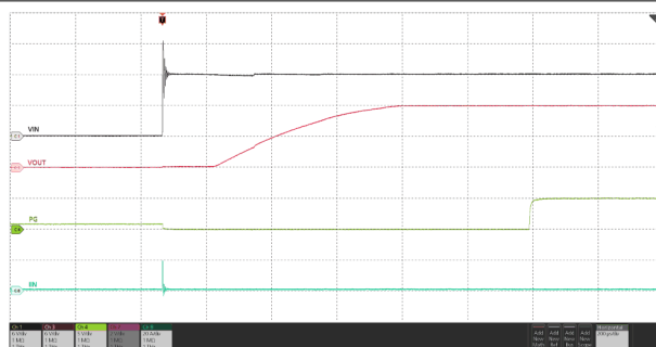
Figure 7-32. Input Hot-Plug
