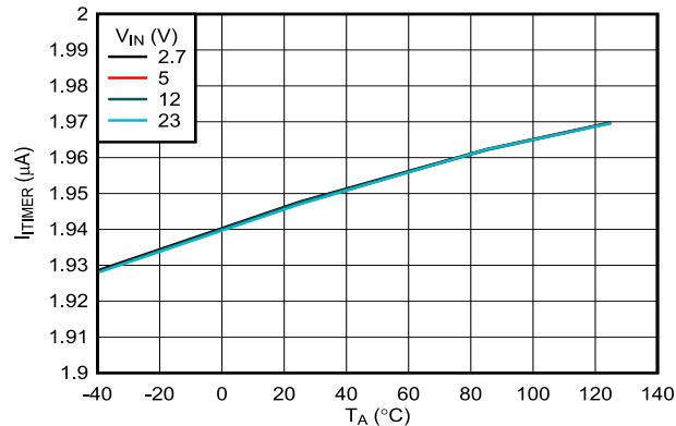
Figure 7-21. ITIMER Discharge Current vs Temperature
