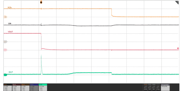
Figure 7-44. Output Short-Circuit During Steady State
