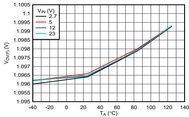
Figure 7-11. OVLO Falling Threshold vs Temperature (TPS25970x, TPS25974x Variants)
