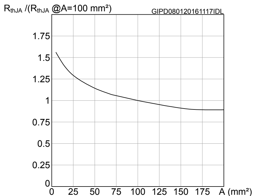
Figure 3. R_{thJA}/(R_{thJA}@A=100\text{ mm}^2)
