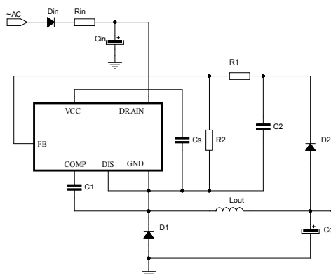
Figure 1. Basic application schematic
