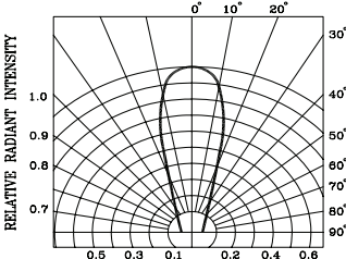
RADIATION DIAGRAM
