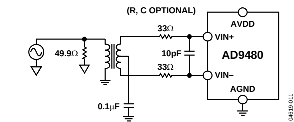
Figure 31. Driving the ADC with an RF Transformer
