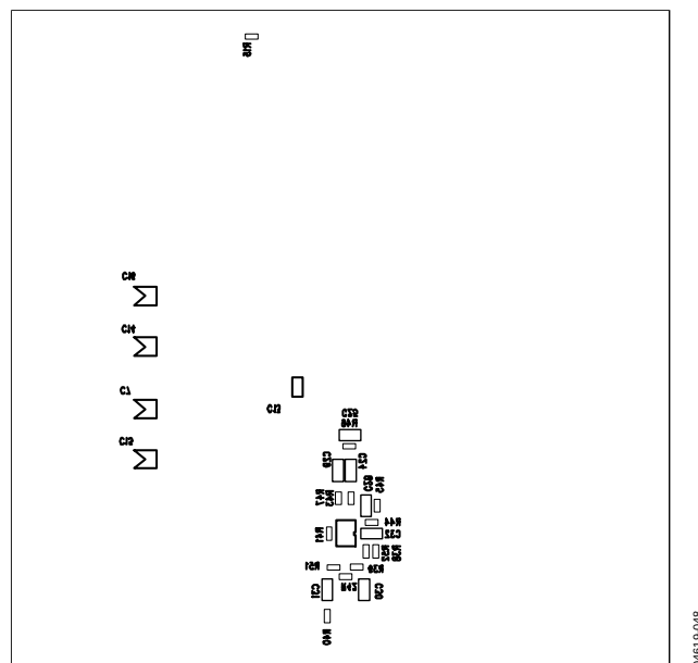
Figure 48. PCB Bottom-Side Silkscreen
