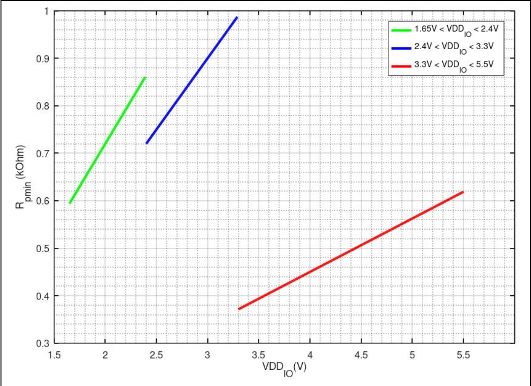
Figure 28. R_{Pmin} vs. V_{DD} , f_c = 3.4 MHz
