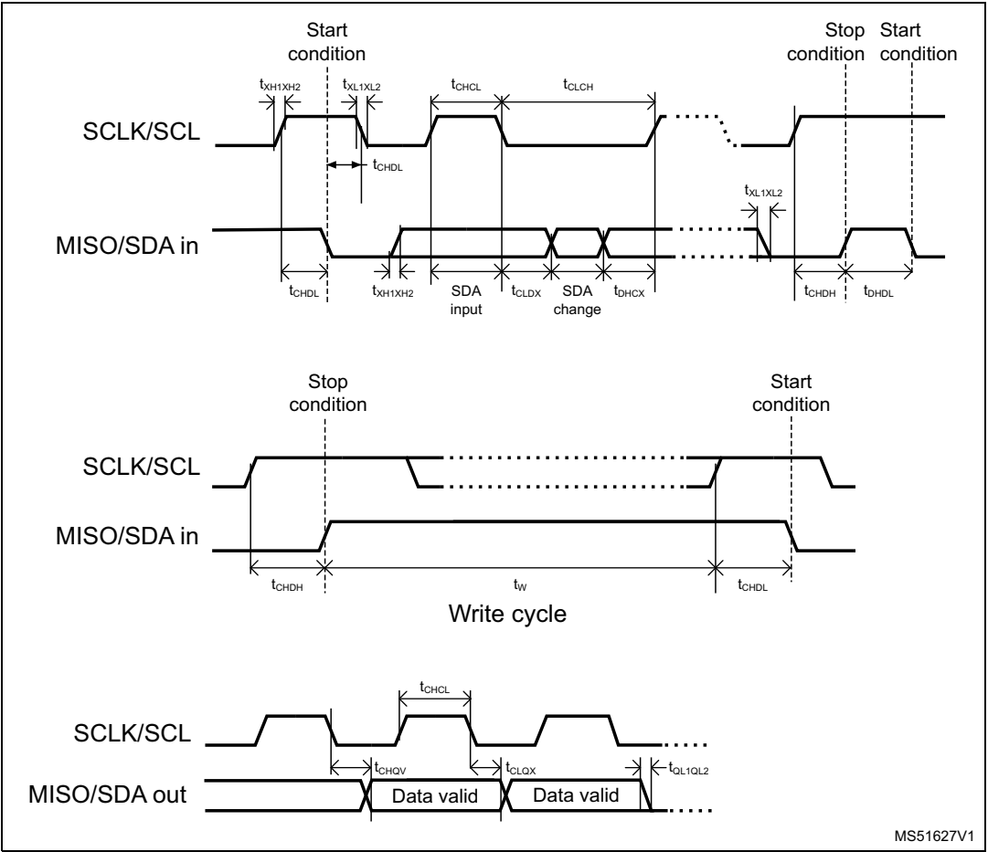
Figure 30. I2C AC waveforms
