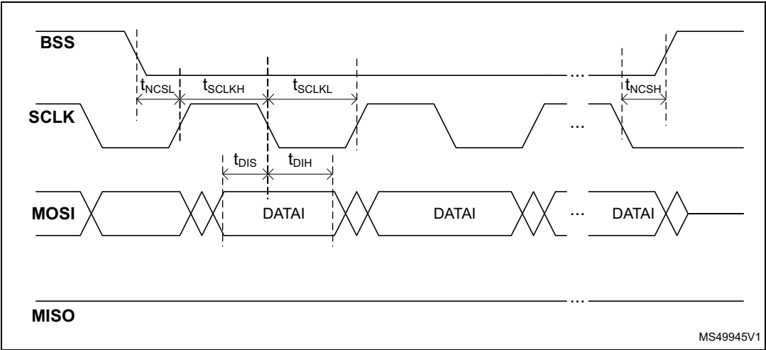
Figure 26. SPI timing diagram - General operation
