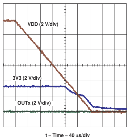
Figure 8-18. Shut Down Behavior at V DD = 12 V (Input Shortened to GND)
