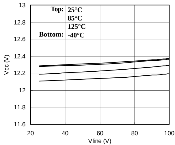
Figure 12 - V cc vs. V line and Junction Temperature
