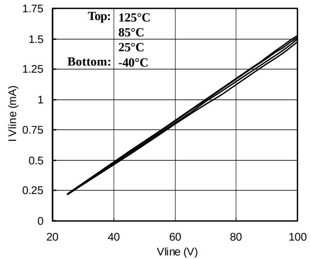
Figure 13 - I(V line ) vs. V line and Junction Temperature
