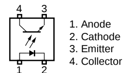
PIN CONNECTION (Top View)
