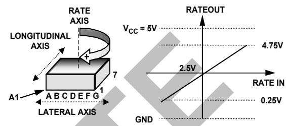
Figure 2. RATEOUT Signal Increases with Clockwise Rotation
