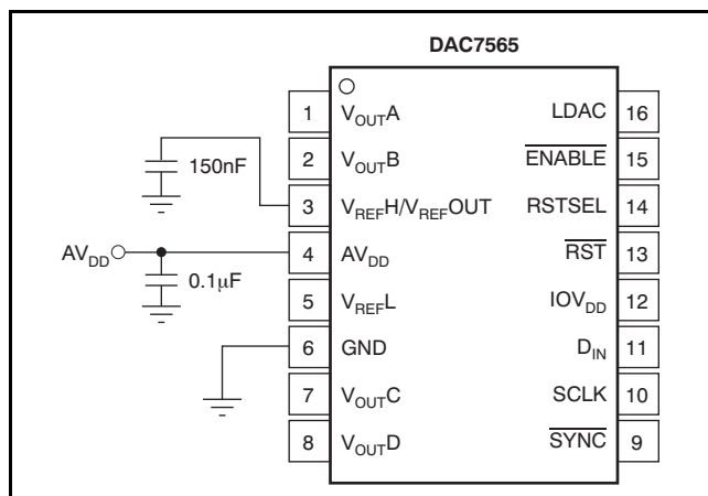
Figure 97. Typical Connections for Operating the DAC7565 Internal Reference
