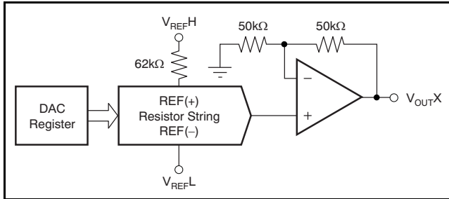
Figure 92. DAC7565 Architecture
