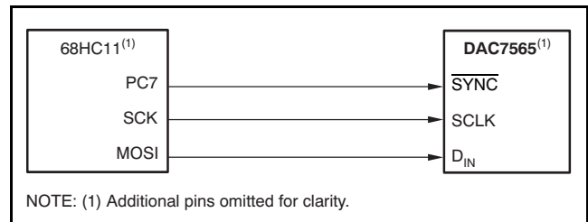
Figure 103. DAC7565 to 68HC11 Interface
