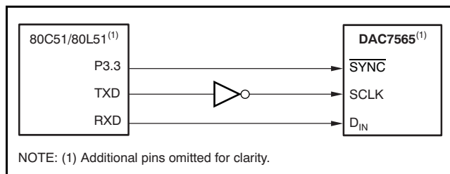
Figure 101. DAC7565 to 80C51/80L51 Interface
