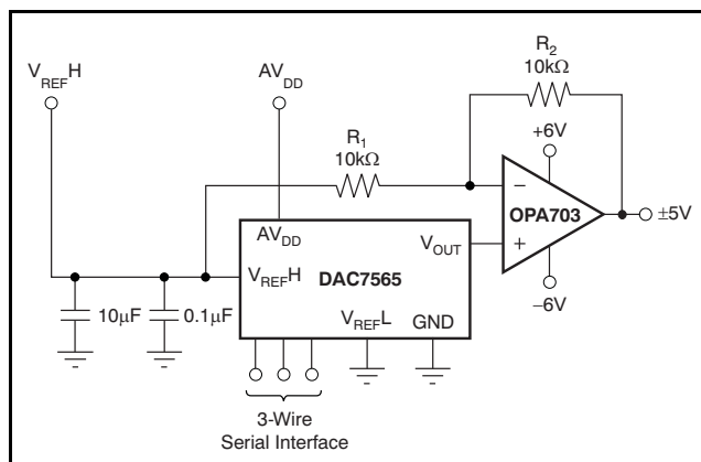
Figure 99. Bipolar Output Range Using External Reference at 5V
