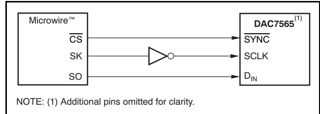
Figure 102. DAC7565 to Microwire Interface
