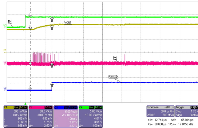
Figure 8. Start up with Prebias Vout, FCCM = Low @ 30mA
