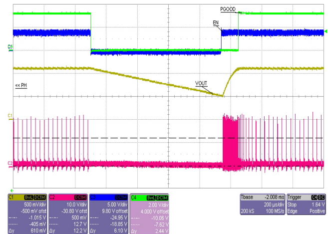
Figure 16. Over Current Protection at 30A
