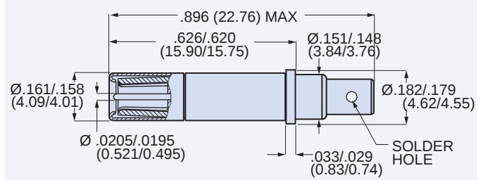
Socket Contact 852-037
