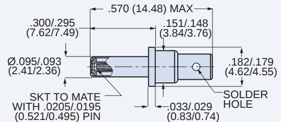
Socket Contact 852-037
