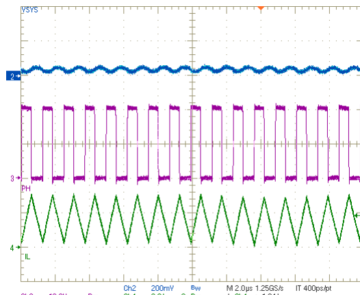
Figure 27. Current Disabled
