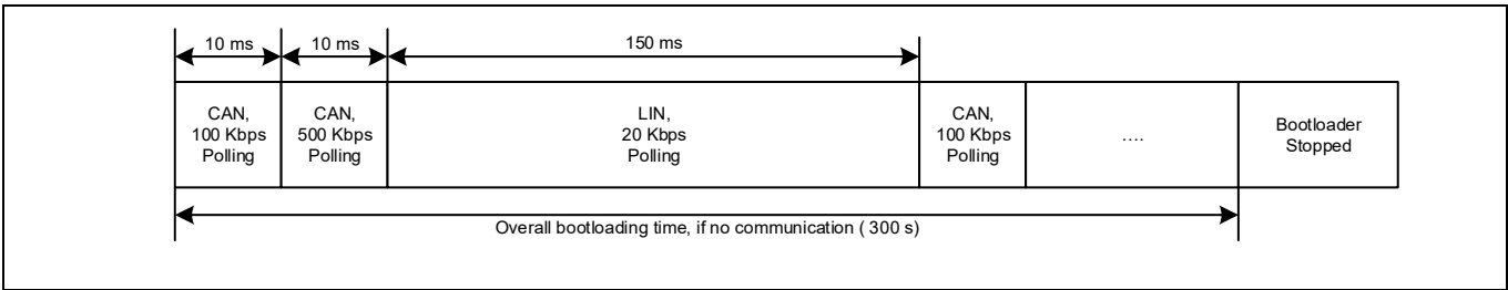
Figure 31-1 Bootloading sequence
