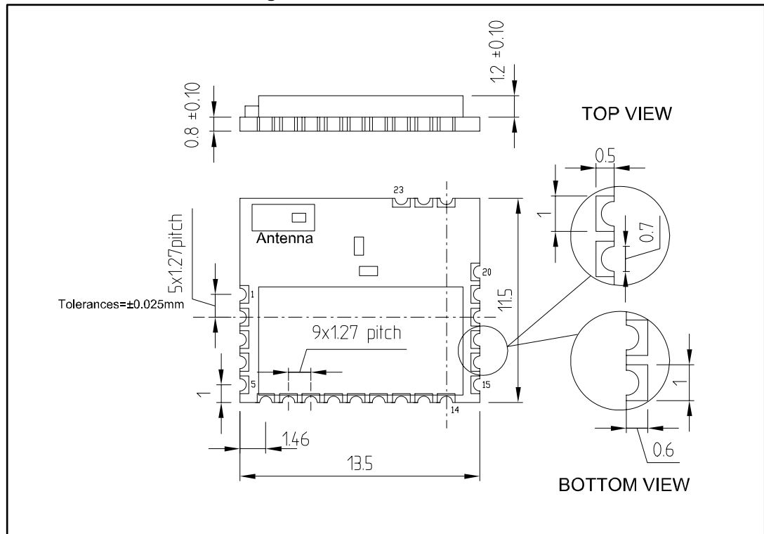
Figure 8: Mechanical dimensions
