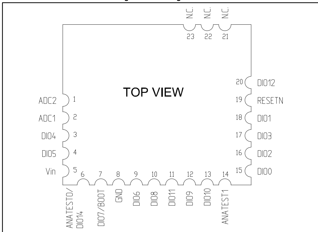
Figure 7: Pin assignment
