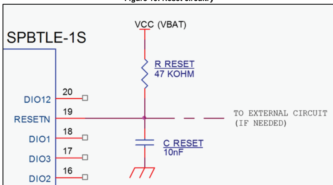
Figure 10: Reset circuitry
