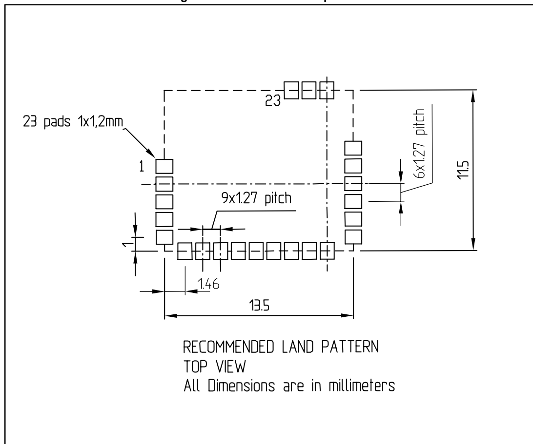
Figure 9: Recommend land pattern
