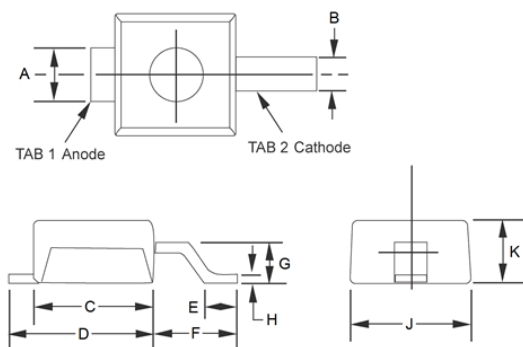
Figure 4-1. Package Dimensions
