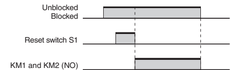
Timing Chart
