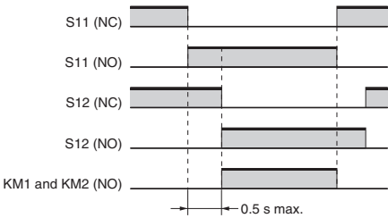
Timing Chart
