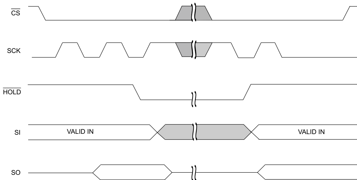
Figure 13. \overline{HOLD} Operation [2]
