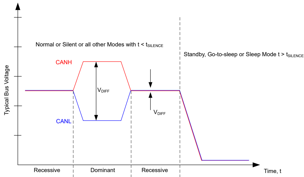
Figure 9-13. Bus States
