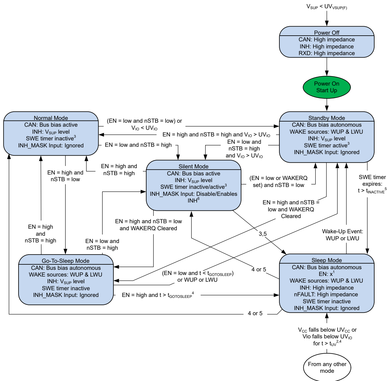
Figure 9-6. TCAN1463-Q1 State Machine
