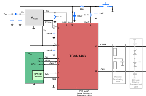
Simplified Schematic
