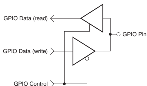
Figure 30. \text{GPIO} Port Pin
