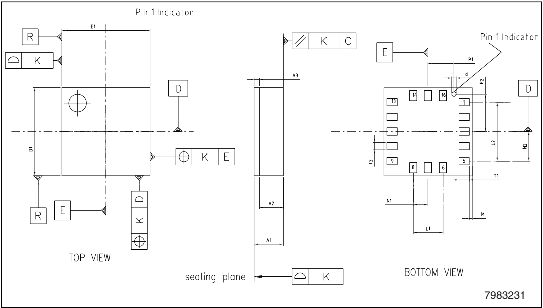
Figure 12. LGA-16: drawing
