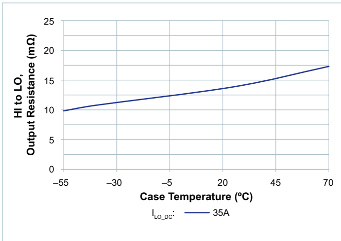
Figure 12 — R_{LO} vs. temperature; nominal V_{HI\_DC} , I_{LO\_DC} = 35\text{A}
