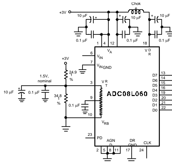
Figure 30. Simple, Low Component Count Reference Biasing
