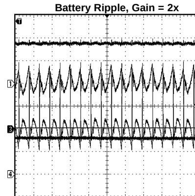
V_{IN} = Li-Ion Battery at 3.7V, Load = 400mA; LED = PWF1; CH1 (MID-TOP): V_{OUT} ; Scale: 20mV/Div, AC Coupled; CH2 (MID-BOTTOM): V_{IN} ; Scale: 50mV/Div, AC Coupled; CH3 (TOP): V_{IN} ; Scale: 1V/Div, DC Coupled; CH4 (BOTTOM): I_{IN} ; Scale: 500mA/Div; Time scale: 1 \mu\text{s} /Div
