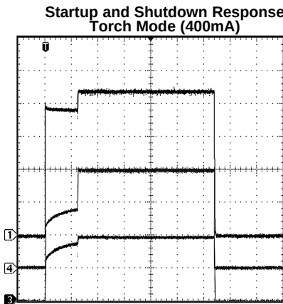
V_{IN} = 3.6\text{V} , Load = 400mA, LED = PWF1; CH1 (TOP): V_{OUT} ; Scale: 1V/Div, DC Coupled; CH4 (MIDDLE): I_{IN} ; Scale: 200mA/Div CH3 (BOTTOM): I_{OUT} ; Scale: 200mA/Div ; Time scale: 100ms/Div
